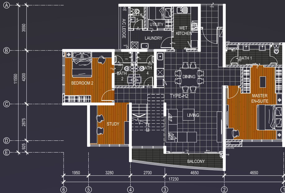
TYPE H2/H3 Lower floor
