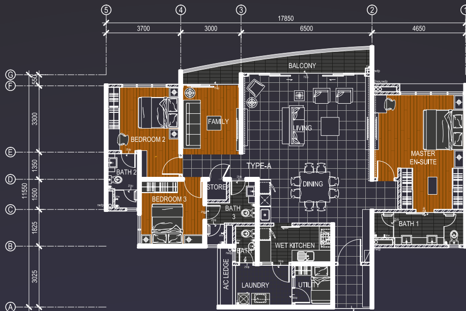
TYPE A/A1
