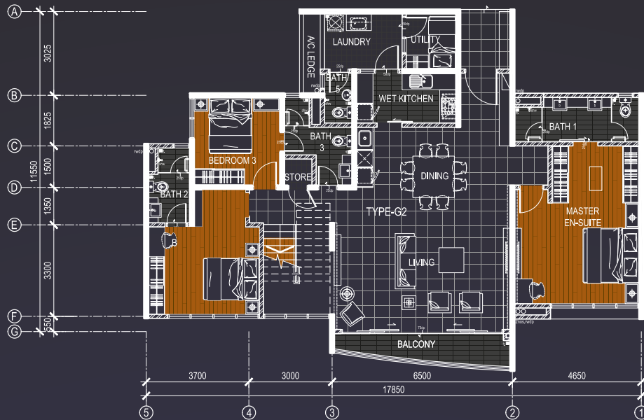
TYPE G2/G3 Lower floor
