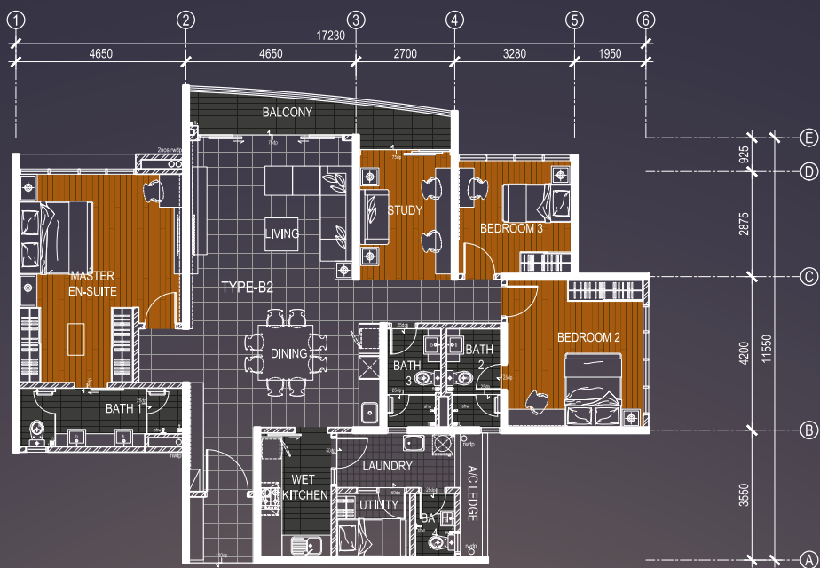
TYPE B2/B3
