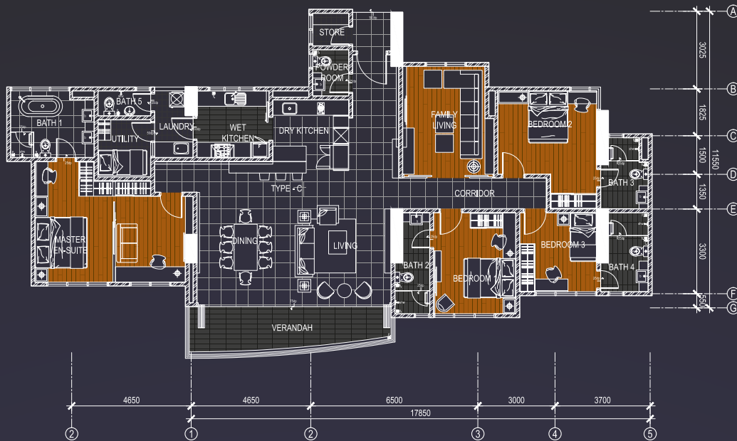
TYPE C/C1
