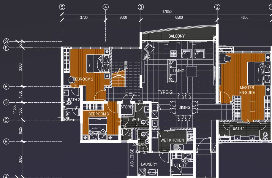
TYPE G/G1 Lower floor
